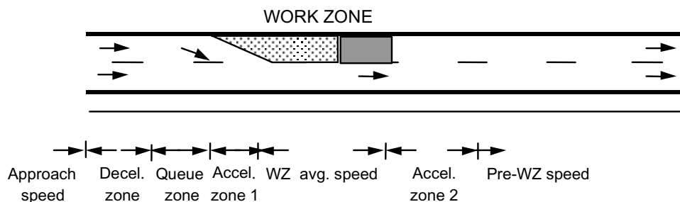
Figure 7.2. Traffic behavior associated with queue formation near a work zone.
