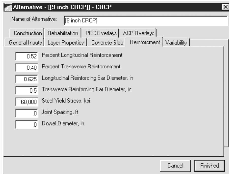
Illustration 9.18. Reinforcement Design.
