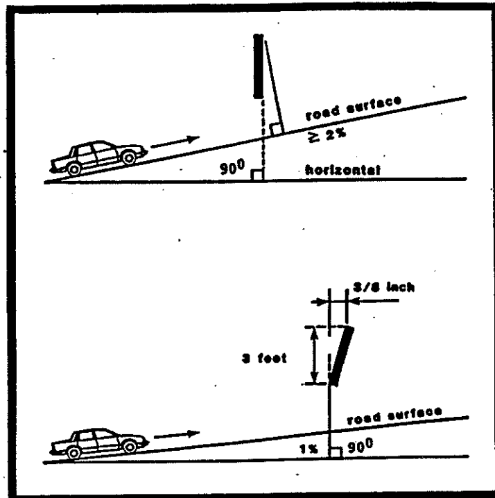
Orientation of Overhead Signs
