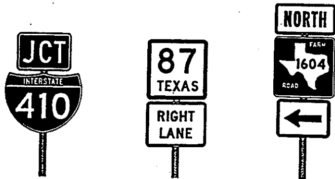
Guide Sign Units
