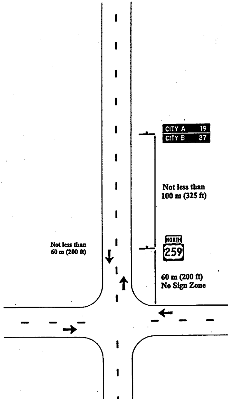
Departure Sign Placement, Guide Signs Beyond the No Sign Zone
