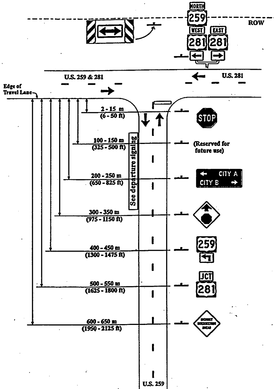
Illustration of Convention for Sign Placement Distances
